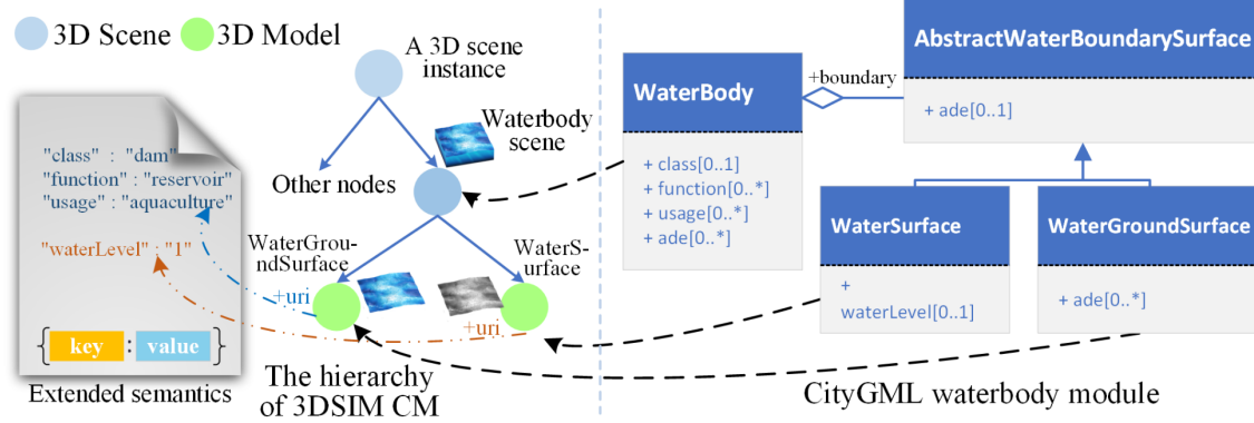
Figure 5. Attribute mapping of the waterbody module in CityGML to a 3D asset described by 3DSIM CM.
