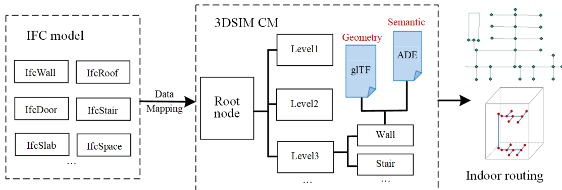
Figure 15. Shortest route planning across multiple stories in a 3D building managed in 3DSIM CM.
