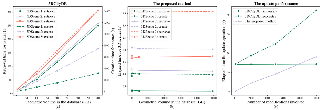
Figure 16. Performance comparison between 3DCityDB and the proposed method:
